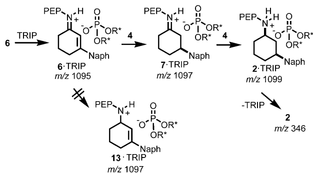
Scheme 3. Formation of ion pair intermediates; m/z ratios refer to protonated species. PEP = p -ethoxyphenyl, Naph = naphthyl.
