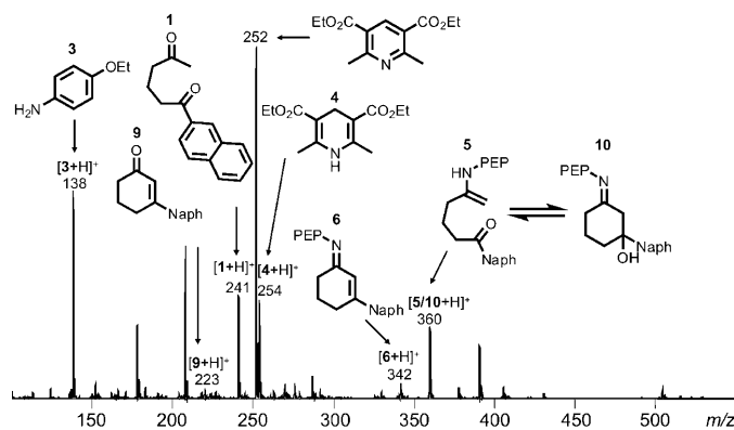
Figure 1. ESI-MS spectrum (positive mode) of the cascade reaction for the synthesis of 3-substituted cyclohexylamines, 5 min after the start of the reaction.
