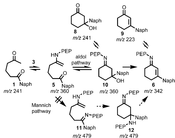
Scheme 2. Plausible and detected intermediates of the aldolization step; m/z ratios refer to protonated species. PEP = p -ethoxyphenyl, Naph = naphthyl.
