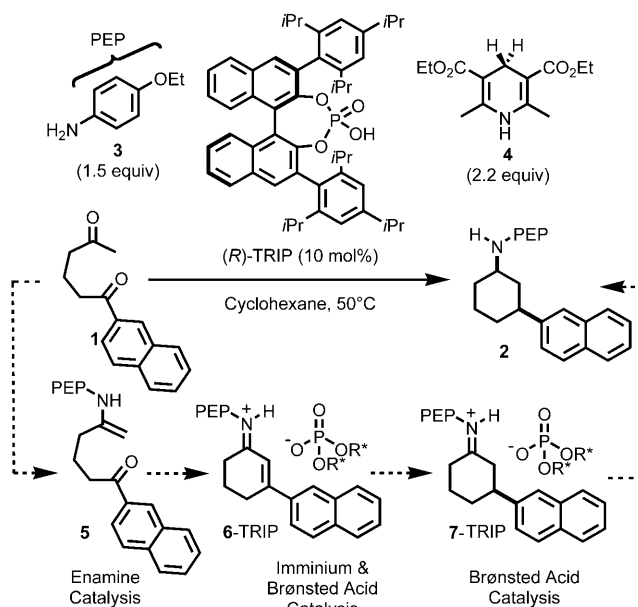
Scheme 1. Quadruple organocatalytic cascade reaction for the synthesis of 3-substituted cyclohexylamines from 2,6-diketones via proposed intermediates. PEP = p -ethoxyphenyl.
