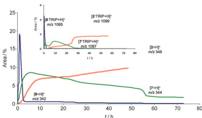
Figure 4. Formation of ions and ion pairs during 80 h of reaction time.
