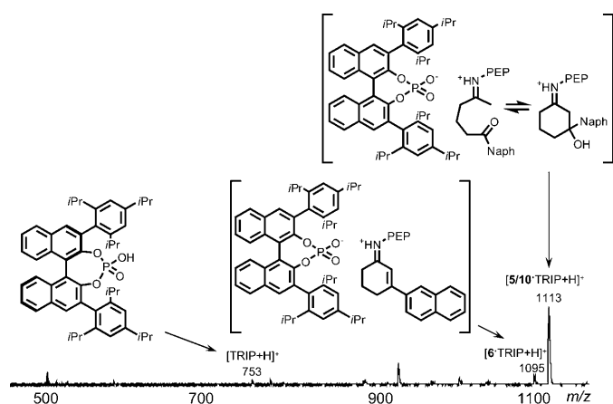
Figure 2. ESI-MS (positive mode) spectrum of the cascade reaction for the synthesis of 3-substituted cyclohexylamines, 5 min after the start of the reaction. Detection of protonated ion-pair intermediates are presented in the spectrum.
